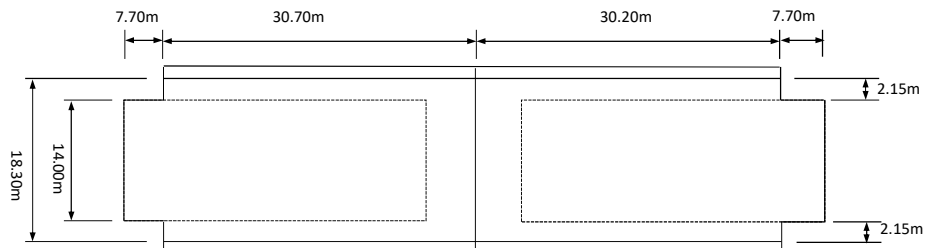
Tank top deck - Uniform load: 11.7Tons/m 2
