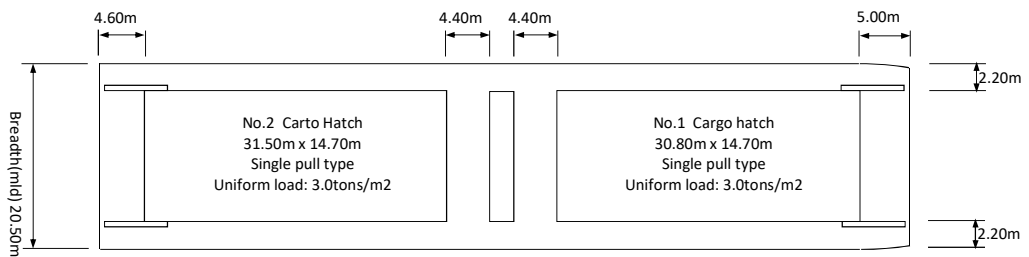
Upper deck/On hatch - Uniform load: 3.0tons/m 2
